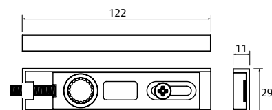
Top Pivot Housing
