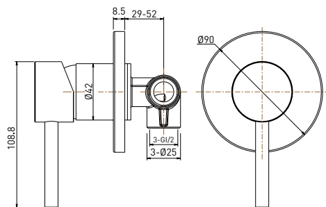
Mixer
