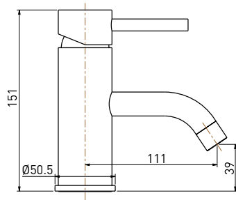
Basin Mixer
