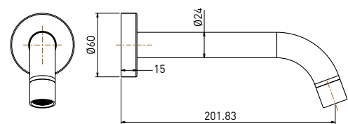
Bath Spout
