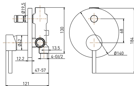
Mixer Diverter
